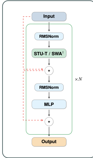
Figure 12: FlashSTU architecture [22].
